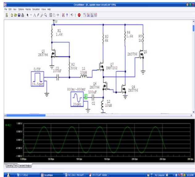
Fig. 7 RF input of simulated mixer with circuit maker 2000
