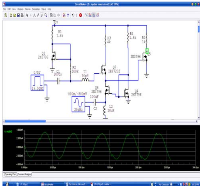
Fig. 8 Output results of simulated mixer
