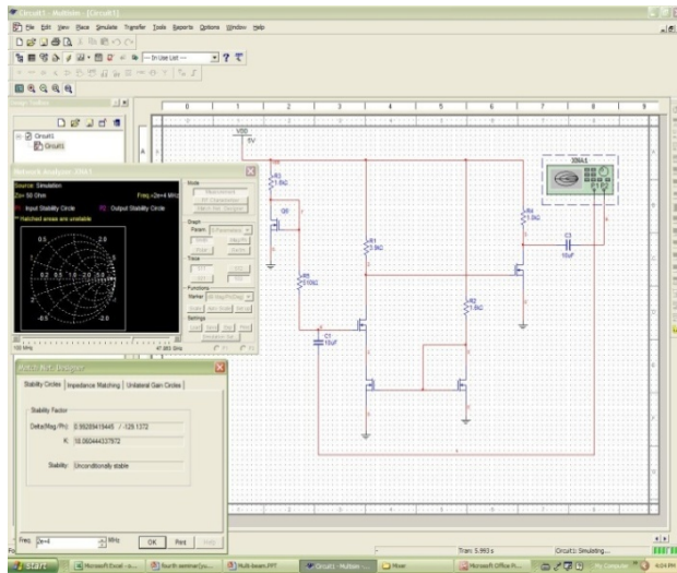
Fig. 4 Stability checking for mixer circuit
