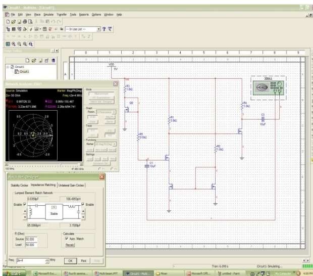
Fig. 5 Impedance matching for mixer circuit
